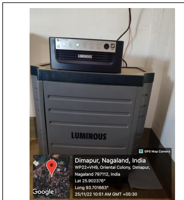
Photograph 4: Installation of 2 KVA inverter in the Seminar Hall
